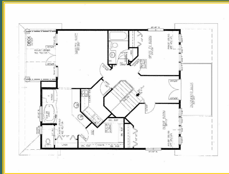
Second Floor Plan @ 1,090
